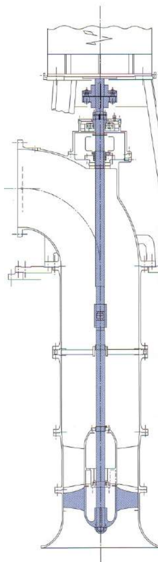
Open line shaft
