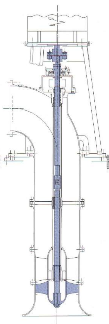
Enclosed line shaft
